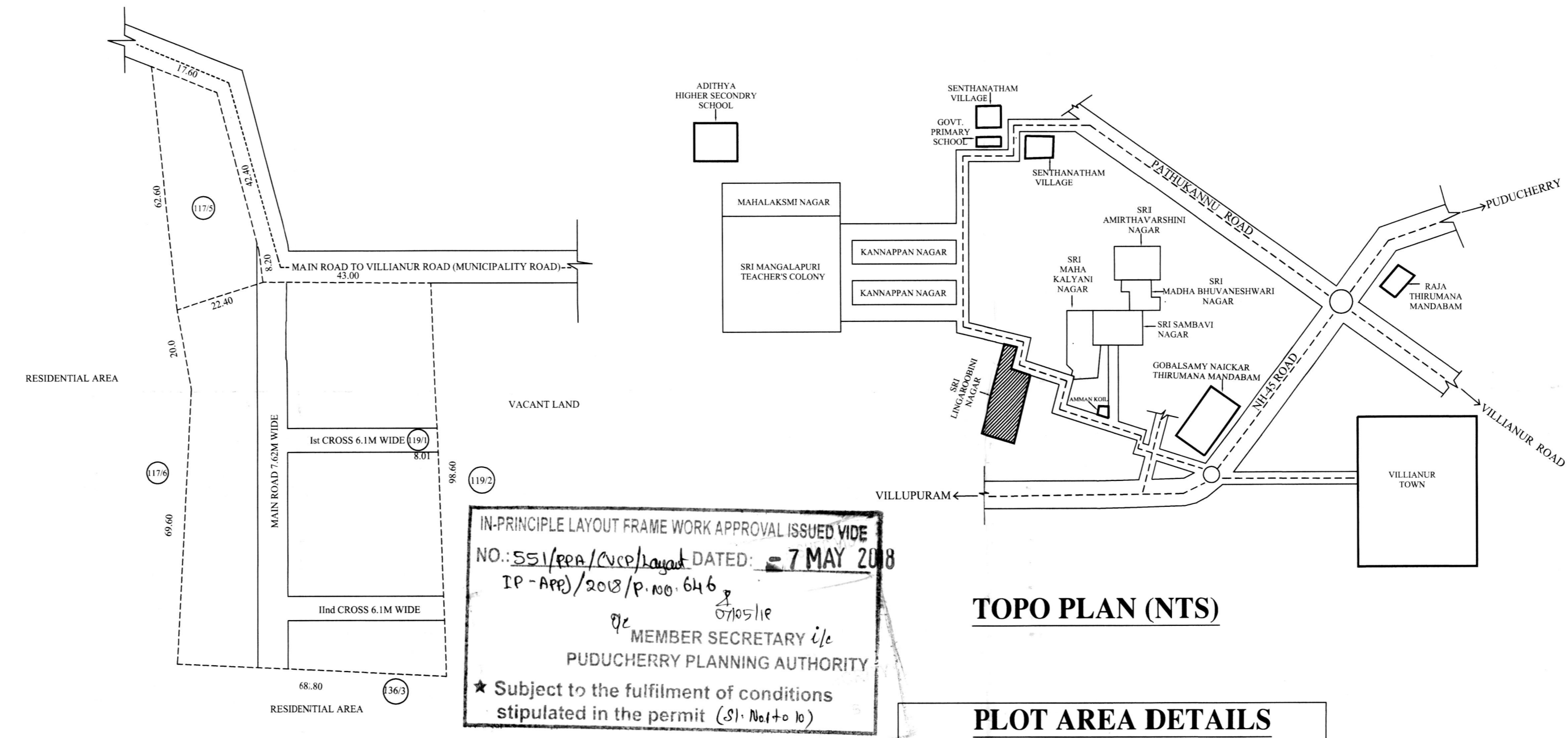
ROAD NETWORK, LAND SUB DIVISION DETAILS & LOCATION PLAN OF THE LAYOUT (1:1000)
