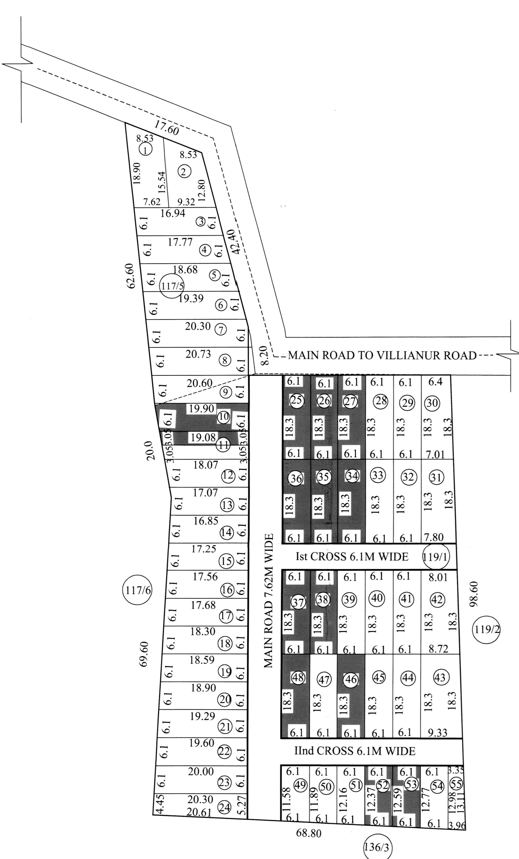
LAYOUT PLAN (1:500)
